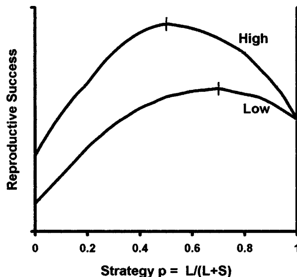
Figure 1 (Baum). Reproductive success as a function of strategy, expressed as proportion of long-term tactics ( L ) relative to long- and short-term ( S ) mating effort overall. The curve labeled "High" shows the possibilities for a more attractive individual. The curve labeled "Low" shows the possibilities for a less attractive individual. Crosses indicate optimal strategies. The optimal strategy for the more attractive individual includes more short-term tactics and is higher overall than that for the less attractive individual.
