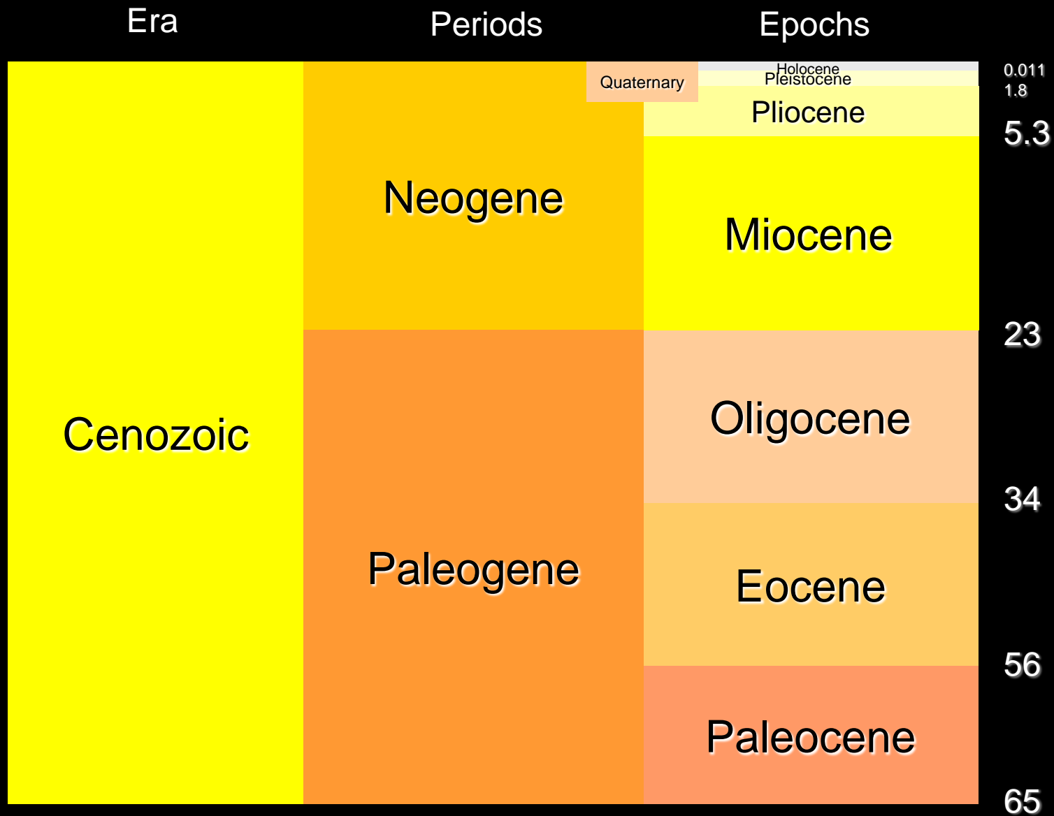
The Cenozoic (drawn to scale)
