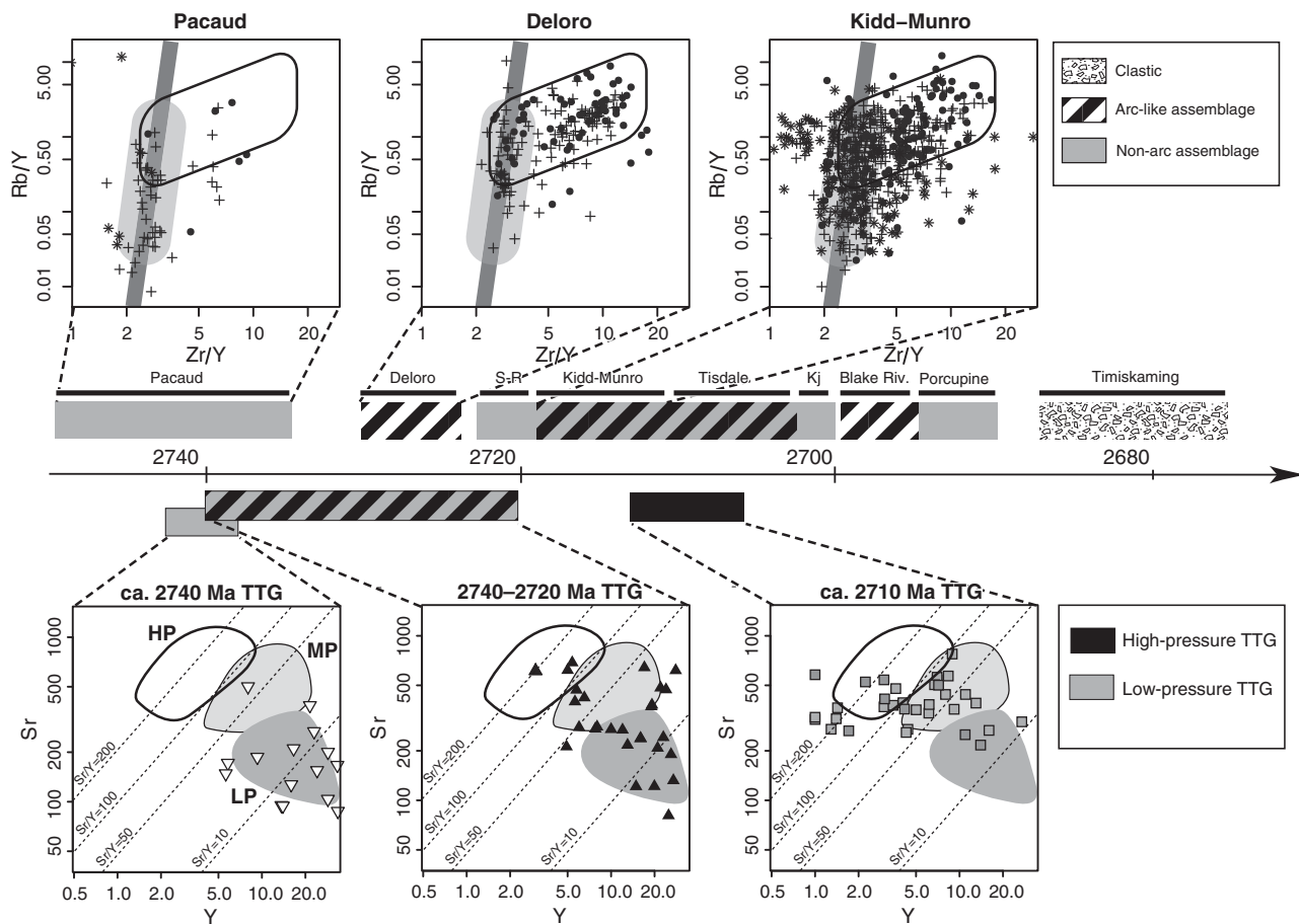
Figure 1. The succession of “arc” and “non-arc” events in the Western Abitibi, Canada (time line, middle, and top legend) is geochemically defined by (1) the nature of mafic ( \text{SiO}_2 < 62\% ) lava assemblages (top; data from http://www.discoverabitibi.com/ , and Ayer et al. [2004]), and (2) concomitant (tonalites, trondhjemites, and granodiorites: TTG) plutons in the Kenogamissi complex, Abitibi greenstone belt (bottom; modified from Benn and Moyen, 2008). For mafic lavas, Rb/Y versus Zr/Y allows us to take into account X-ray fluorescence analyses from the database that lack a whole set of trace elements; Th/Yb versus Nb/Yb (see the Data Repository [see footnote 1]) show the same pattern. Symbols reflect the major element characteristics of the samples, based on Jensen (1976) classification: circles—calc-alkaline; crosses—komatiitic; stars—tholeiitic. The main criteria used to classify an assemblage as “arc” or “non-arc” are (1) the position in these diagrams (omitting outliers); (2) the presence or absence of komatiites; and (3) the existence of intermediate to acid calc-alkaline lavas (not plotted here). (See details in Benn and Moyen, 2008; Kerrich et al., 1999a; Kerrich et al., 1999b; Sproule et al., 2002; Wyman, 2003; Wyman et al., 2002). Three examples (the “non-arc” Pacaud, the “arc” Deloro, and the “mixed” Kidd-Munro assemblage) are displayed; see Appendix DR1 (see footnote 1) for the whole stratigraphy. For plutonic rocks, the age determinations are slightly less precise and do not allow a perfect fit with the supracrustal stratigraphy. The ca. 2710 Ma plutons (synchronous with subduction-related lavas in the greenstone belt stratigraphy) belong to the low-HREE (high rare earth element), high-pressure group defined by Halla et al. (2009) and Moyen (2011), and are geochemically clearly different from older TTG. They are synchronous with the emplacement of the Kidd-Munro and Tisdale assemblages, which do contain an “arc” component. In contrast, ca. 2740 Ma low-pressure TTGs occur at the same time as the non-arc Pacaud assemblage. In between, the long-lived Gogama gneisses contain both low- and high-pressure components, and cover a time period corresponding to both the “arc” Deloro period, and the “non-arc” Pacaud.
