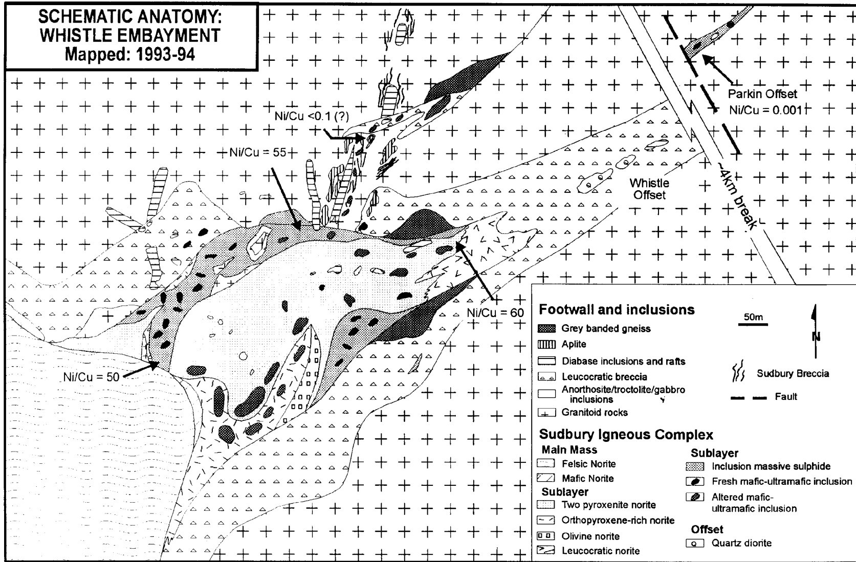
Figure B1. Diagrammatic representation of geological relationships at Whistle Mine (after Lightfoot et al. 1997A,B,C).
