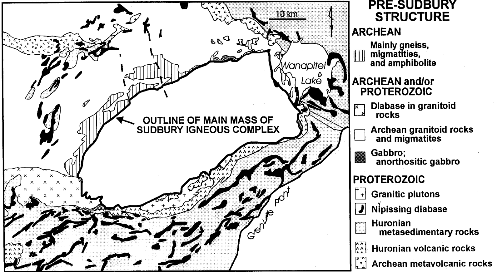
Figure 1. B) Country rocks surrounding the SIC (after Muir, 1984).
