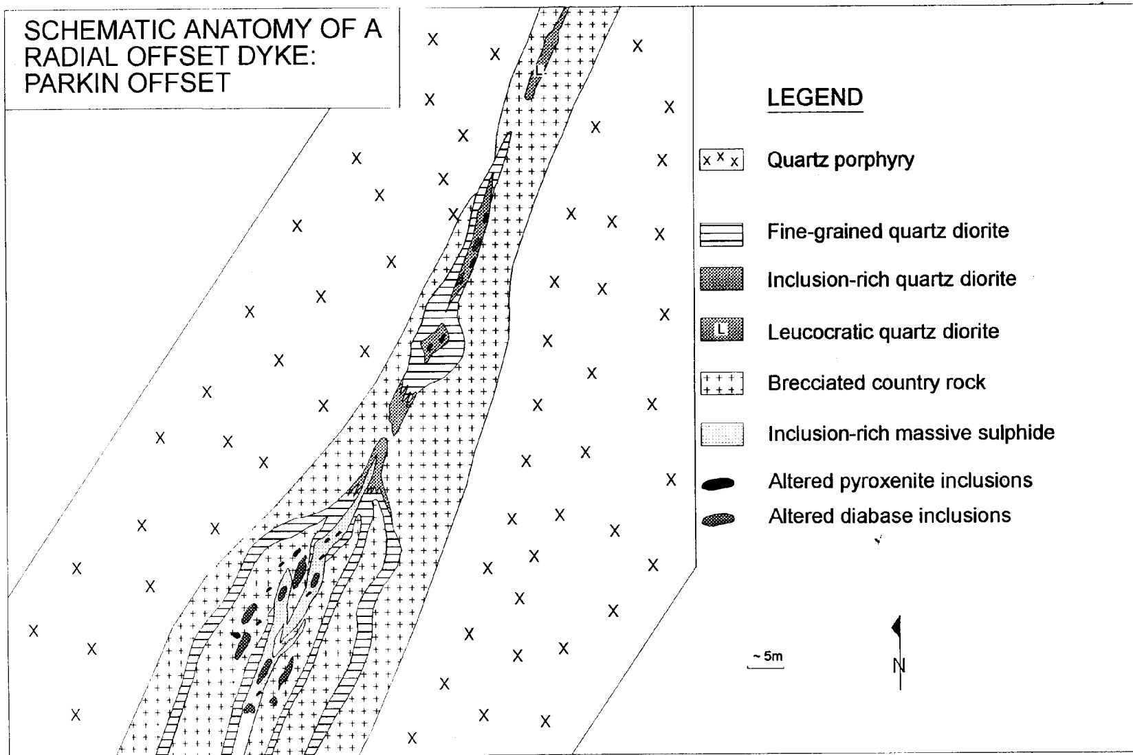
Figure B2. Diagrammatic representation of relationships in the Parkin Offset (after Lightfoot et al. 1997A).
