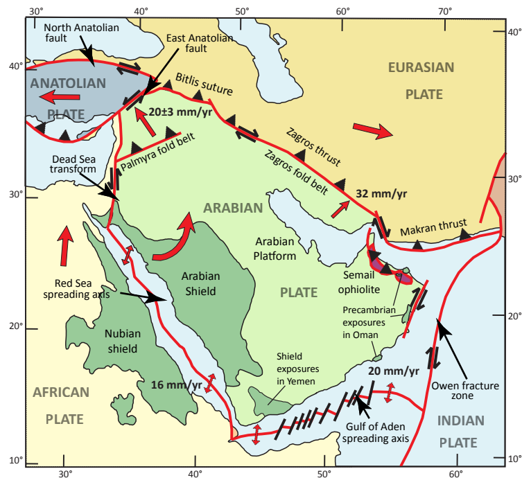
Fig. 1-1. Tectonic setting of the Arabian plate showing its boundaries, rates of drift, and kinematic interactions with adjoining plates. Red arrows show the senses of trajectories of the Arabian and adjacent plates, and rates of movement.
