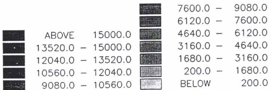
Figure 3. Cumulative area map for Booro-Borotou with a grid spacing of 12.5 m
