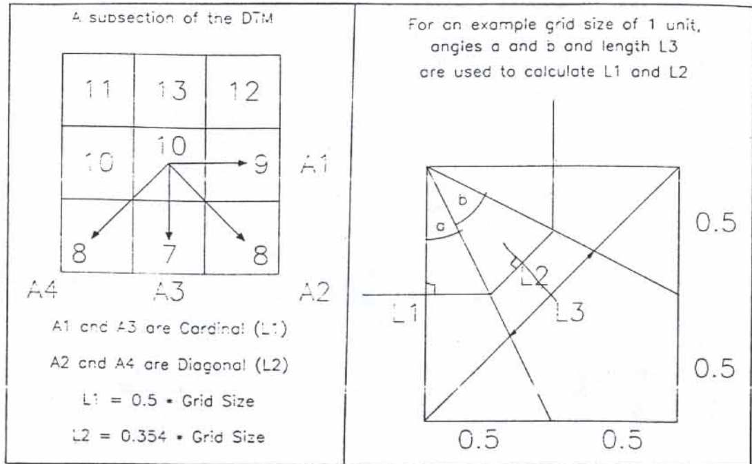
Figure 1. Flow partitioning using the multiple flow direction algorithm
