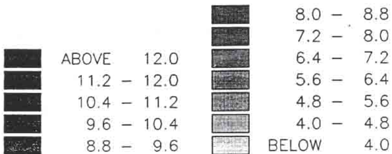
Figure 6. \text{Ln}(a/\tan \beta) map derived using a single flow direction algorithm, with a grid spacing of 12.5 m
